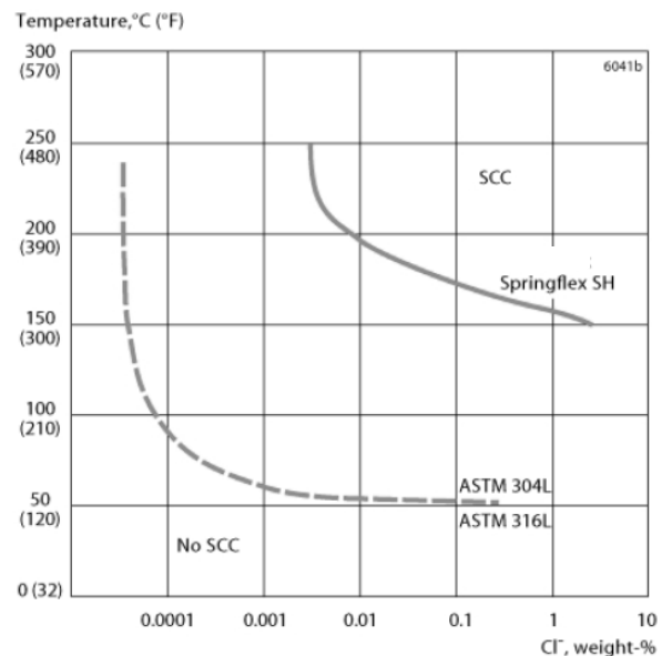
Figure 8. Resistance to stress corrosion cracking, laboratory results for Springflex™ SH of constant load specimens loaded to 85 % of the proof strength at the test temperature.
