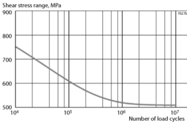
Wöhler diagram, mean stress 450 MPa
