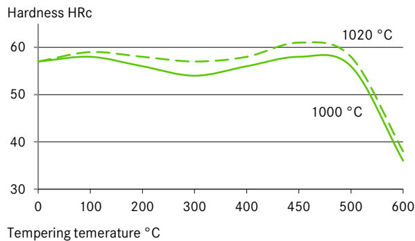
Tempering Chart (Hardening with Subzero Refrigeration)
