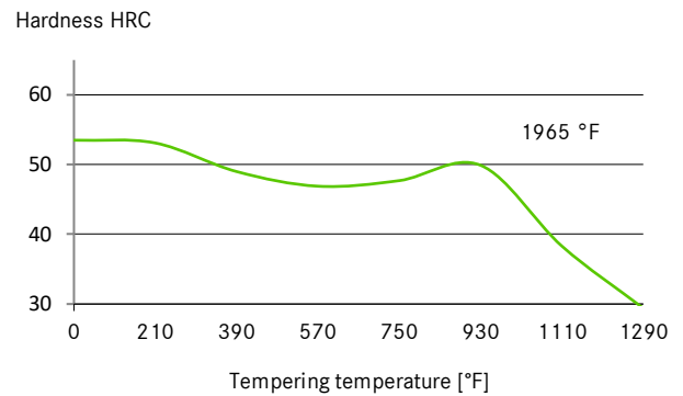
Tempering Chart
